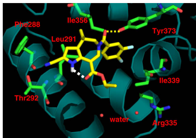
Figure 2. The docked binding mode of 10a (in yellow) in the binding pocket of the hFXR X-ray co-crystal structure (from a complex with 1 ). Only critical residues within the binding site have been shown for clarity. Hydrogen bonds are shown by dotted lines (white intramolecular, yellow intermolecular).
