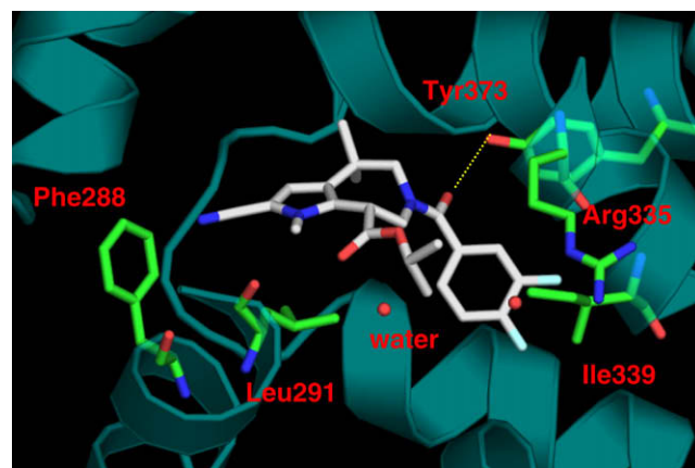
Figure 3. The docked binding mode of 11a (in white) in the binding pocket of the hFXR X-ray co-crystal structure (from a complex with 1 ). Only critical residues within the binding site have been shown for clarity. Hydrogen bonds are shown by dotted yellow lines. The ester carbonyl group is now twisted out of plane and not in position to form hydrogen bond with NH of pyrrole.
