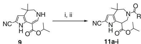
Scheme 2. Reagents and conditions: (i) NaCNBH 4 , AcOH, 20 °C, 61%; (ii) RC(O)Cl, Et 3 N, CH 3 CN, 20 °C, 80%.
